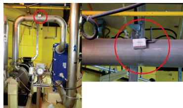
(a) Primary loop pump and output pipe.
