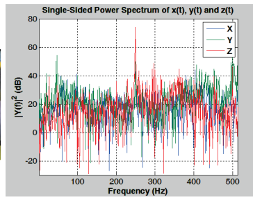
(b) Vibration Power spectrum.
