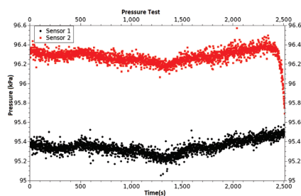
(b) Pressure measurement.
